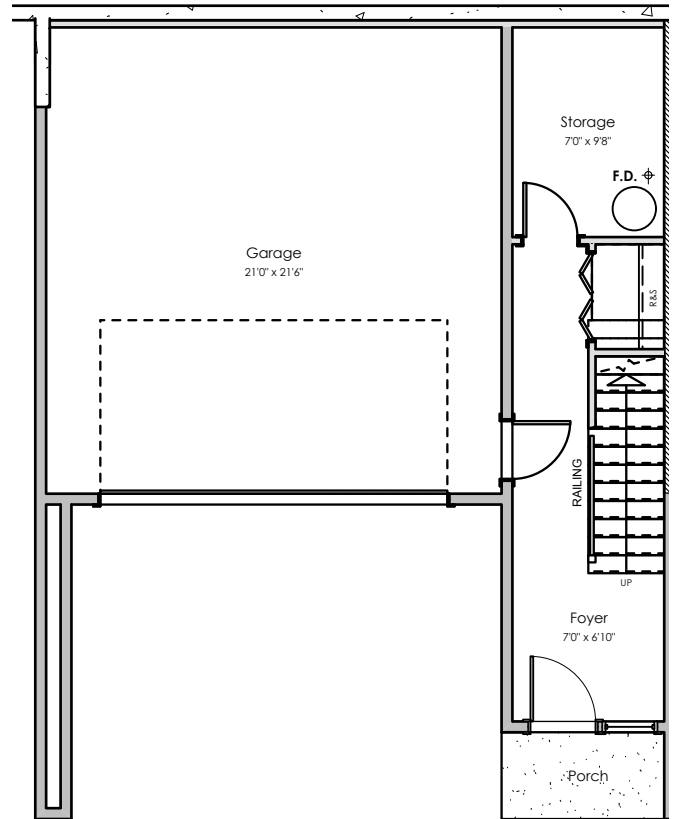
LOWER FLOOR 247 SQ FT
