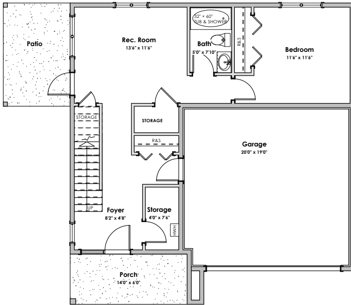
LOWER FLOOR 642 SQ FT
