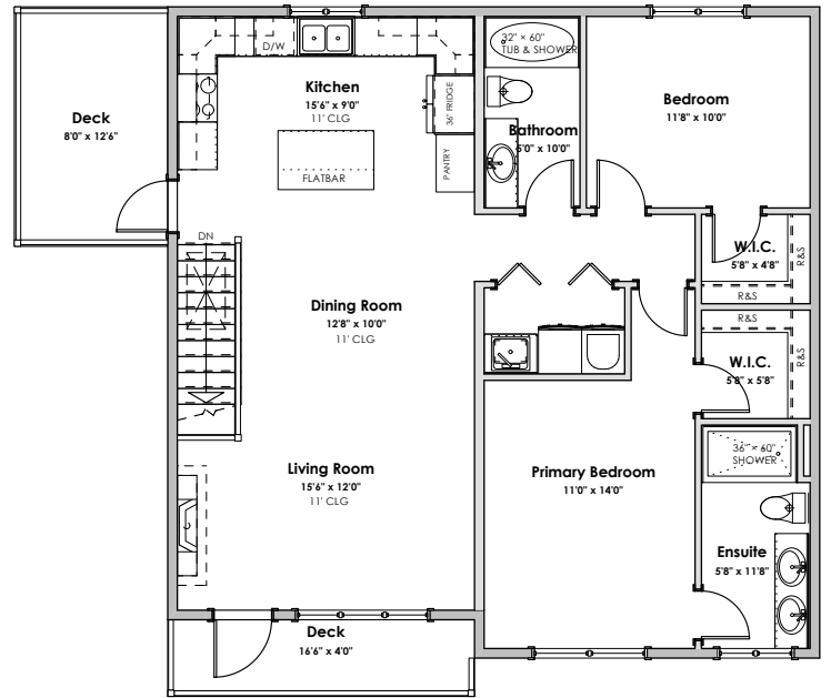
UPPER FLOOR 885 SQ FT
